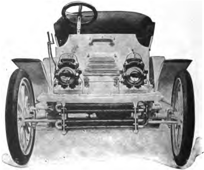
FIG. 410.—Front view of "Peerless" Tonneau Carriage, showing the radiating coils and bonnet for covering the motor; inclined steering pillar with hand-wheel and control levers at the right of the driver's seat.
